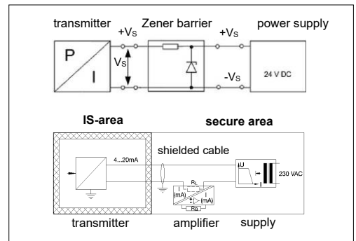
Fig. 3 circuit diagrams
